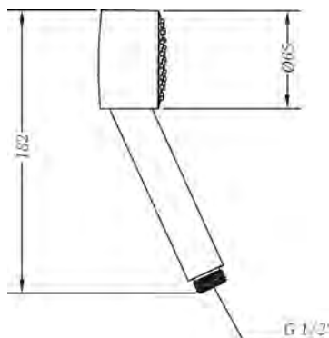
Ref.: 100197 45 00 Mango de ducha C1 jet (bolsa) C1 jet handshower (bag)
