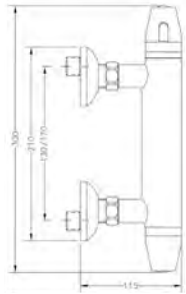
Ref.: 67104 14 45 67 Termostática ducha Thermostatic shower
