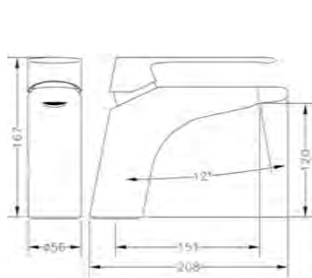
Ref.: 62130 08 45 66 Monomando de lavabo Single lever wash-basin mixer
