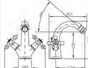
Ref.: 68516 09 43 66 Monobloc bidet bronce Bidet mixer bronze
