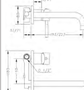
Ref.: 65132 18 45 66 Monomando de lavabo empotrado caño 22cm Built-in wash-basin mixer 22 cm spout
