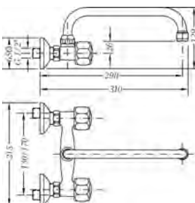
Ref.: 68193 11 45 66 Grupo mural fregadera 15 cm caño tubo alto 24cm Wall sink mixer 15 cm with high tube spout 24 cm
