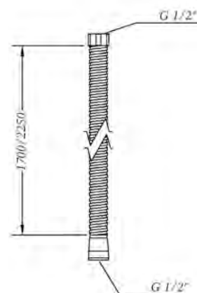
Ref.: 100137 60 00 Flexo extensible 1,70 - 2,25 m inoxidable doble grapaje Extendible stainless steel flexible hose 1,70 to 2,25 m double lock
