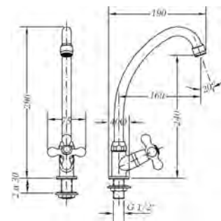
Ref.: 68585 09 45 66 Grifo fregadera vertical caño tubo Sink tap with tube spout
