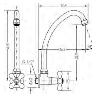
Ref.: 68575 09 45 66 Grifo fregadera mural caño tubo vertical Wall sink tap with goose neck spout
