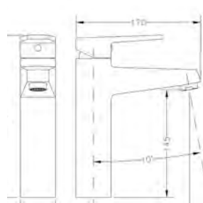
Ref.: 64134 16 45 66 Monomando de lavabo medio alto Medium high single lever wash-basin mixer
