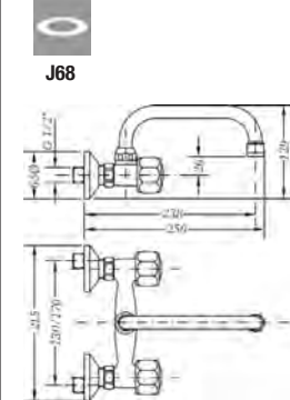
Ref.: 68190 11 45 66 Grupo mural fregadera 15 cm caño tubo alto 18 cm Wall sink mixer 15 cm with high tube spout 18 cm
