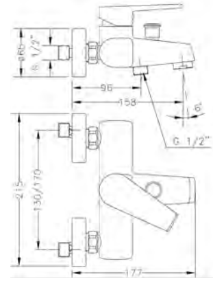
Ref.: 64100 04 45 66 Monomando de baño con kit Single lever bath mixer with kit
