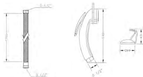
Ref.: 100141 Flexo 1,20m. inoxidable Stainless steel flexible hose 1,20 m.
