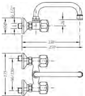
Ref.: 68195 11 45 66 Grupo mural fregadera 11 cm caño tubo alto 18cm Wall sink mixer 11 cm with high tube spout 18cm
