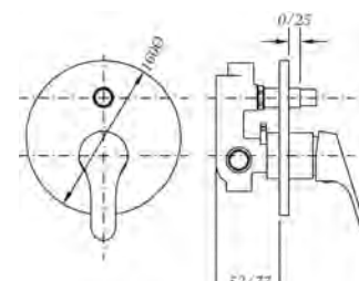
Ref.: 61116 22 45 66 Monomando de baño empotrado con inversor Built-in single lever bath with diverter
